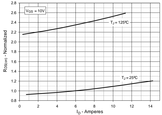
Fig. 4. R_{DS(on)} Normalized to I_D = 6A Value vs. Drain Current
